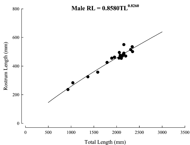
FIGURE 6. Relationship between total length (TL) and rostrum length (RL) in female (n=37) and male (n=22) Pristis microdon .
