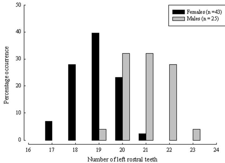
FIGURE 7. Percentage occurrence of the number of left rostral teeth in female and male Pristis microdon .
