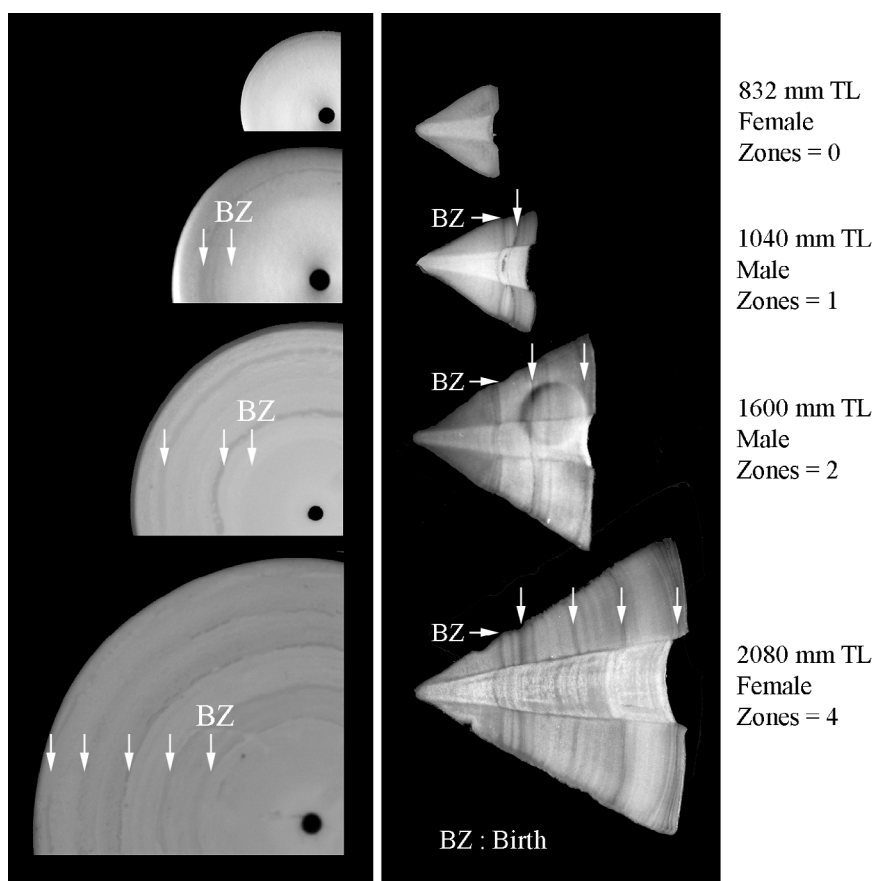
FIGURE 4. Whole and sectioned vertebrae of Pristis microdon , depicting main translucent zones, which are believed to be laid down annually (see text).
