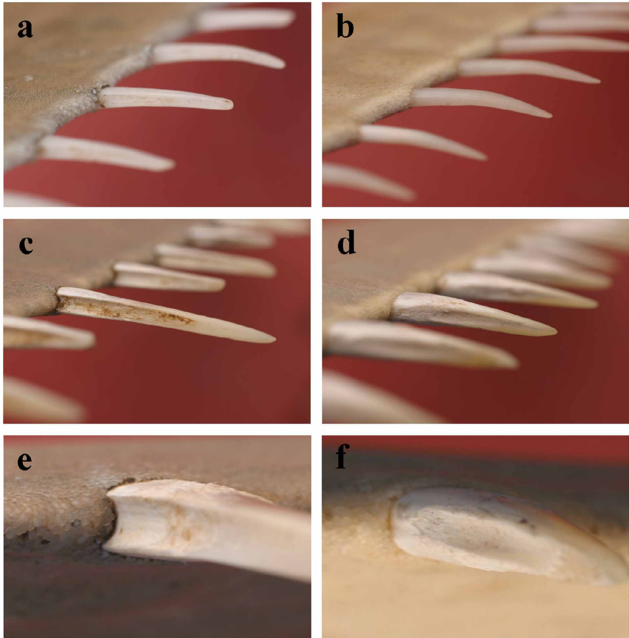
FIGURE 9. Comparison of the rostral tooth shape of Pristis microdon and Pristis clavata from the Fitzroy River, illustrating the strong groove present along the posterior edge of the rostral teeth of P. microdon . This groove is present in (a) small juvenile (832 mm TL) and (c and e) larger juvenile (2271 mm TL) P. microdon , and runs the entire length of the tooth back into the rostrum itself. In comparison, the posterior edge of the rostral teeth of (b) small juvenile (865 mm TL) P. clavata is convex (lacking a groove), and although a groove may be present in (d and f) larger juveniles (2130 mm TL) it is rarely present along the entire length of the tooth.
