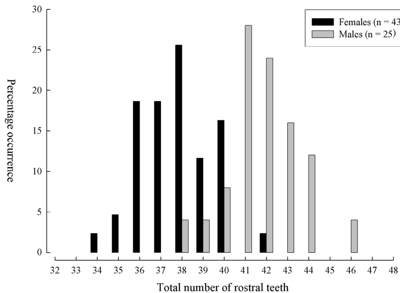
FIGURE 8. Percentage occurrence of the total number of rostral teeth in female and male Pristis microdon .
