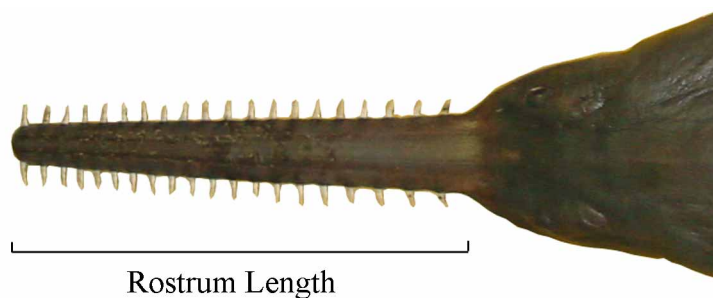
FIGURE 2. Measurement of the rostrum length (RL).
