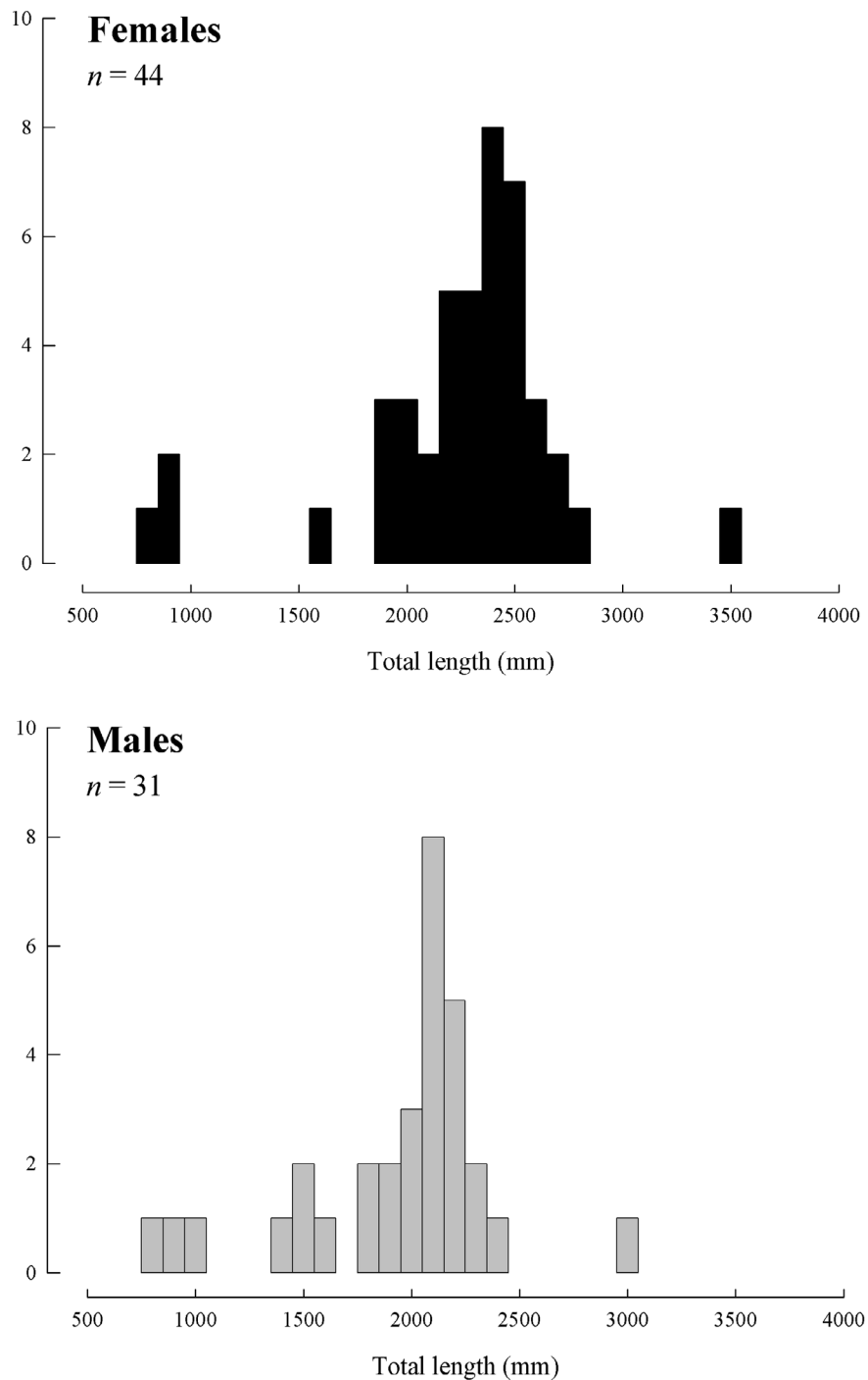
FIGURE 5. Length-frequency histograms for female and male Pristis microdon collected during the study.
